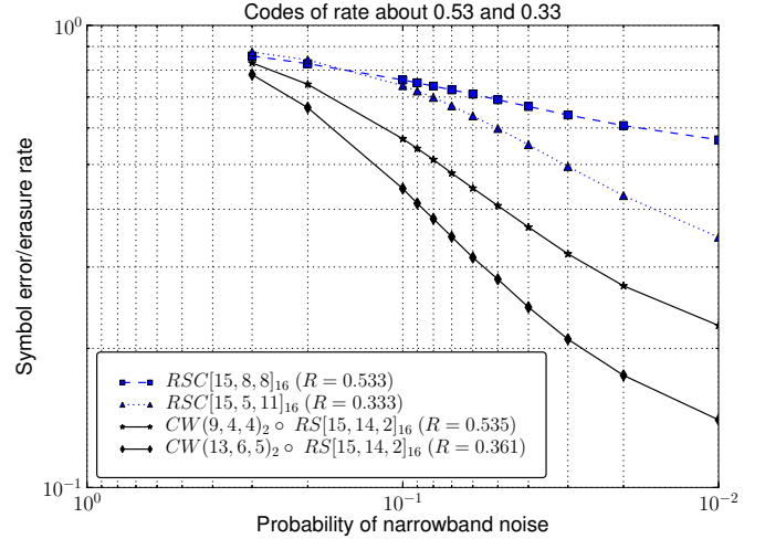
Fig. 1. Comparing concatenated and Reed Solomon codes of similar rates
